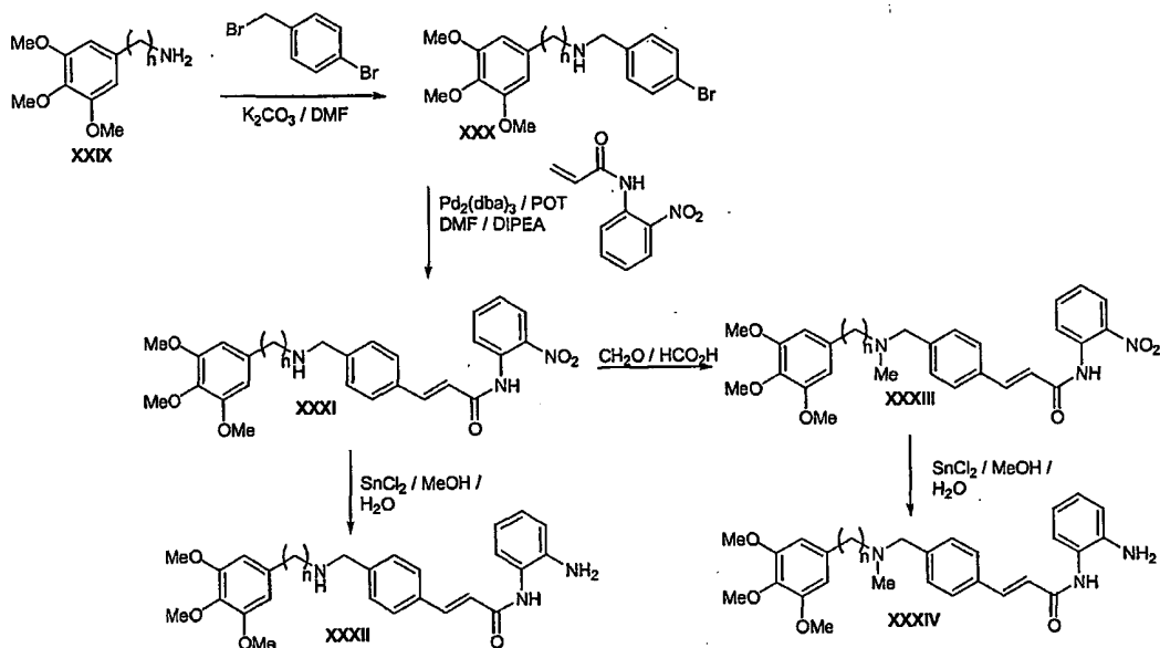
Scheme 5
